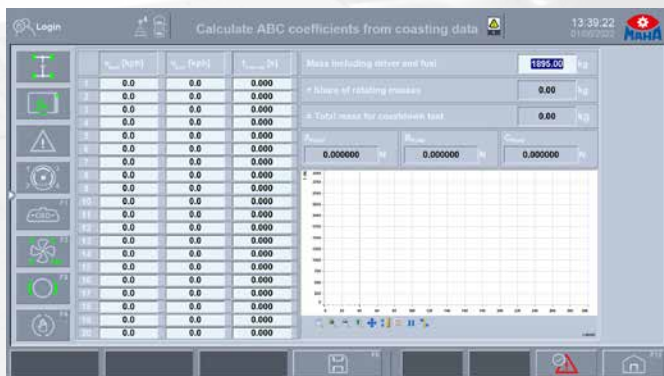
Calculation of ABC coefficients from the vehicle's roll-out data on the dynamometer
