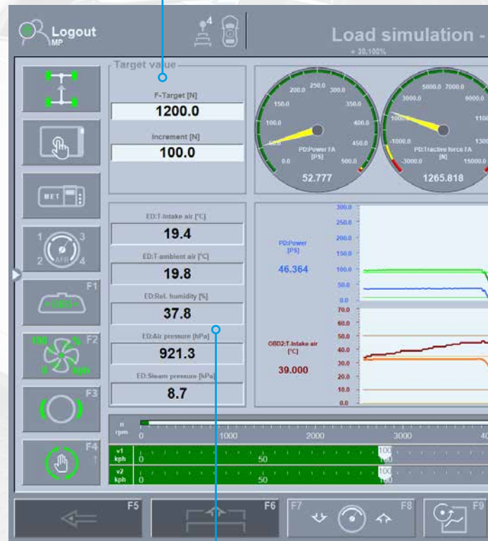
Reference setting dependent on type of load simulation
