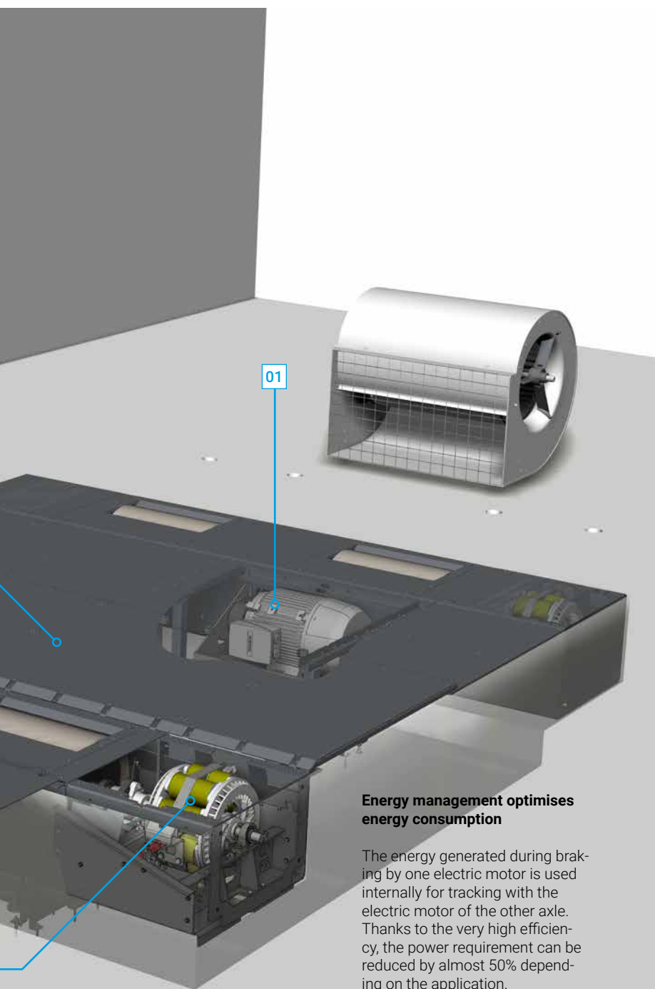
Hydraulic roller set displacement Wheelbase 2.2 m – 3.4 m, infinitely and stably adjustable. The optimised e-motor positioning makes it possible to install in existing MAHA dynamometer foundations without having to adapt the foundation.
