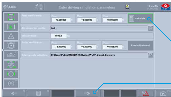
Load adjustment with determination of the dynamometer coefficients. The vehicle's real values can be used and transmitted to the dynamometer
