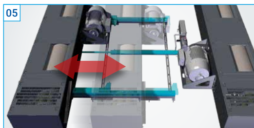
Hydraulic roller set displacement Wheelbase 2.2 m – 3.4 m, infinitely and stably adjustable. The optimised e-motor positioning makes it possible to install in existing MAHA dynamometer foundations without having to adapt the foundation.
